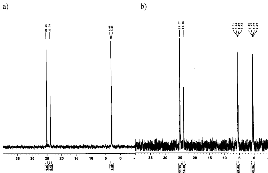
FIGURE 4 ^{31}\text{P} NMR spectra of linear diguanylic acid H-phosphonate 10 . a) ^1\text{H} decoupled; b) ^1\text{H} undecoupled.
