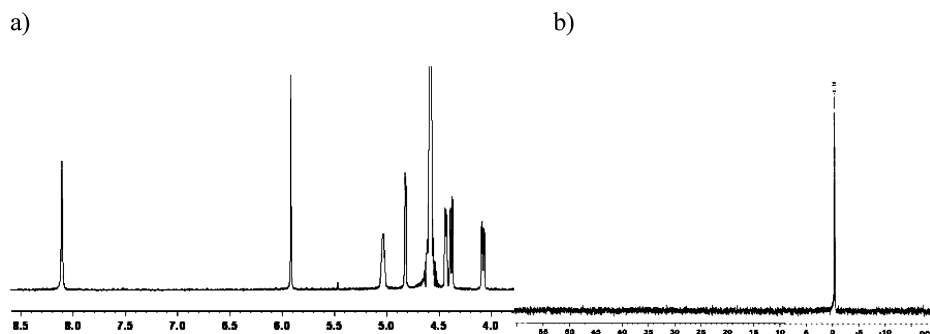
FIGURE 5 a) ^1\text{H} (recorded at 40^\circ\text{C} ) and b) ^{31}\text{P} NMR spectra of the fully-deprotected cdiGMP 15 in \text{D}_2\text{O} .
